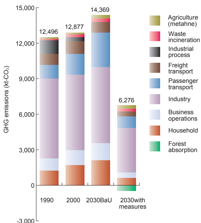
Greenhouse gas emissions
